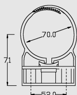
Art. CLC70 (Staffa in nylon Ø 68/70 mm)
